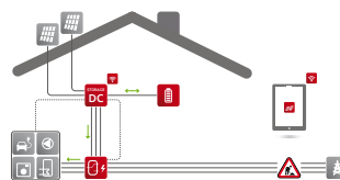
DC STORAGE SYSTEM 4.0 | 6.0 | 8.0 | 10.0 RCT POWER STORAGE DC RCT POWER BATTERY RCT POWER SENSOR RCT POWER SWITCH
