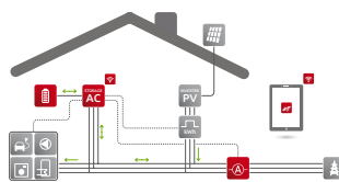
AC STORAGE SYSTEM 4.0 | 6.0 RCT POWER STORAGE AC RCT POWER BATTERY RCT POWER SENSOR
