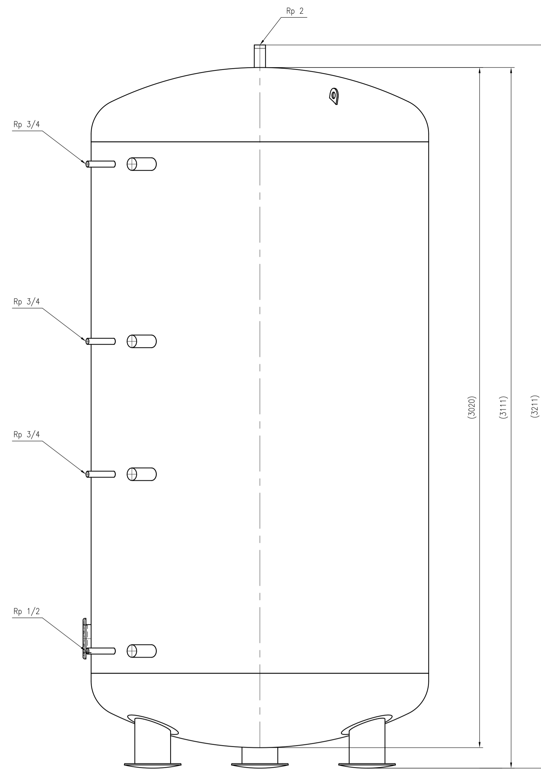
Side view
