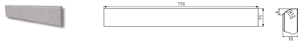
sokl | skirting plinth | DSA89... | 798×95×10 mm
