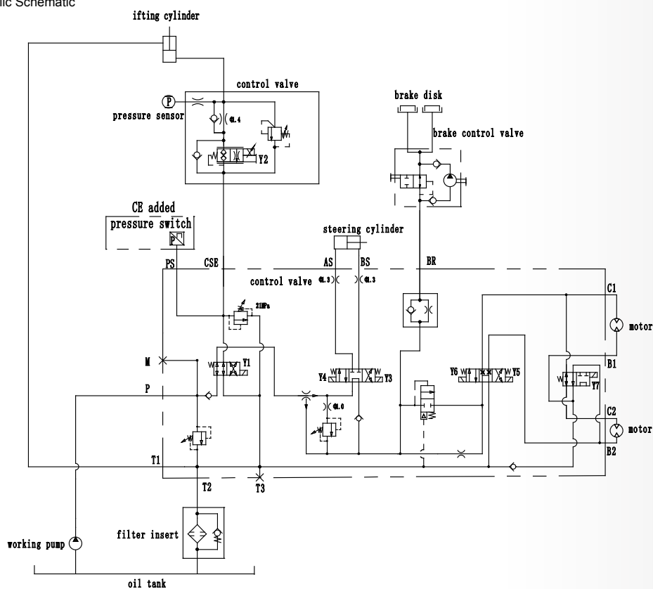
AS0808 Hydraylic Schematic
