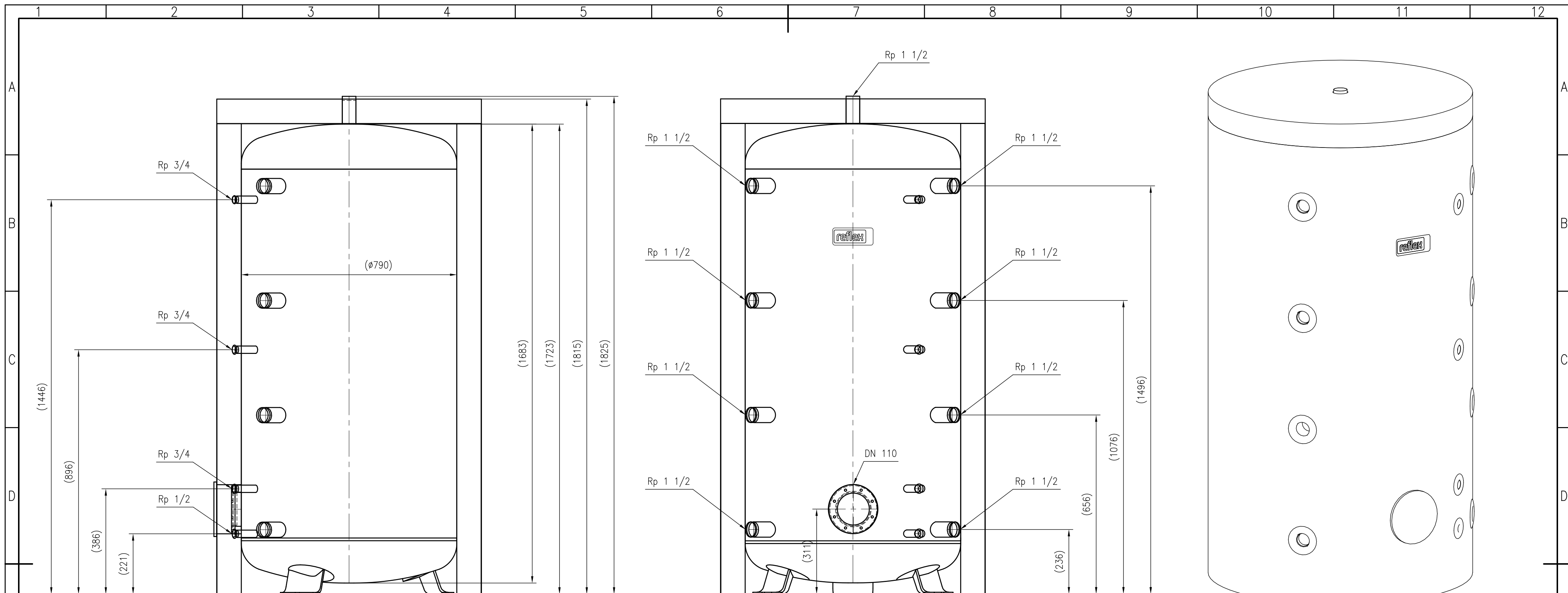
Side view
