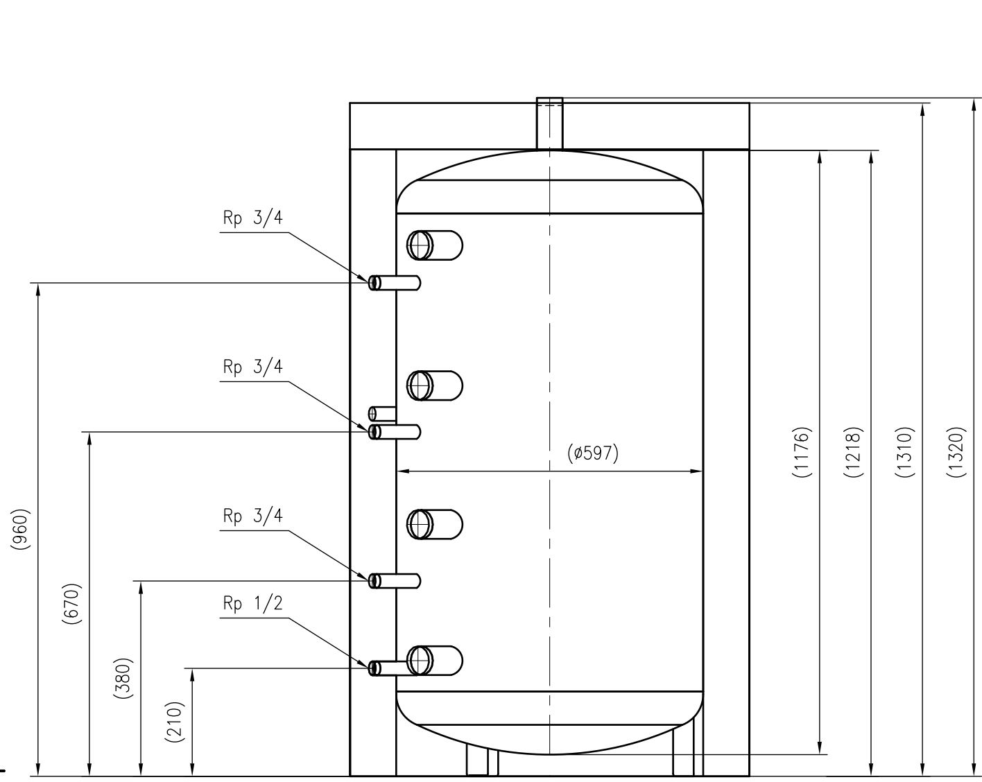
Side view
