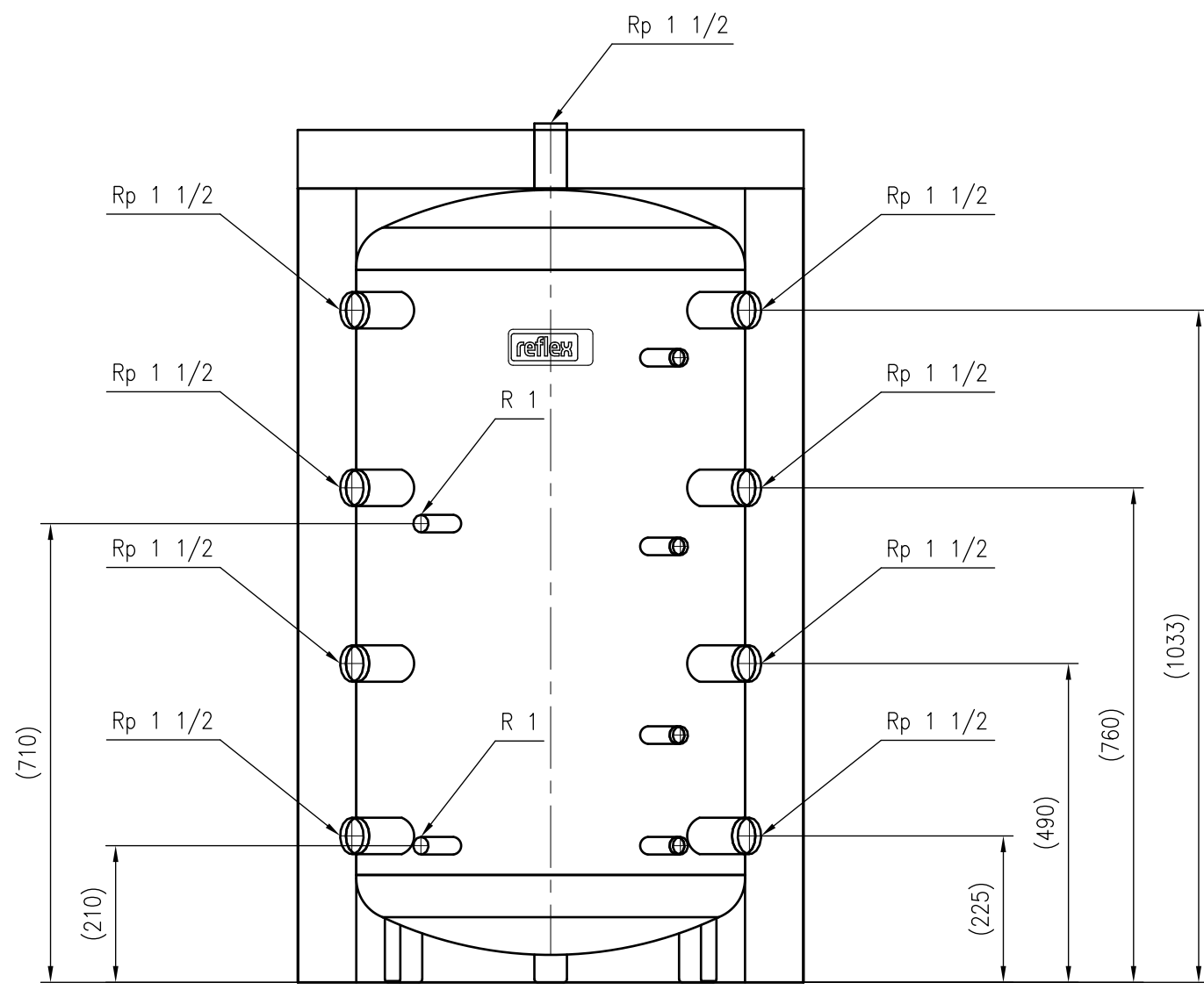
Front view
