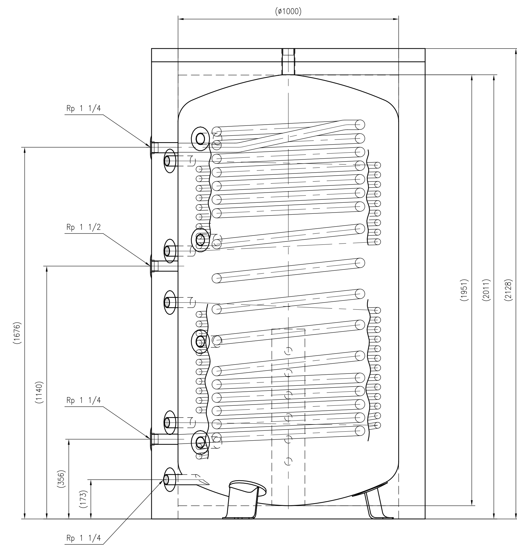
Side view
