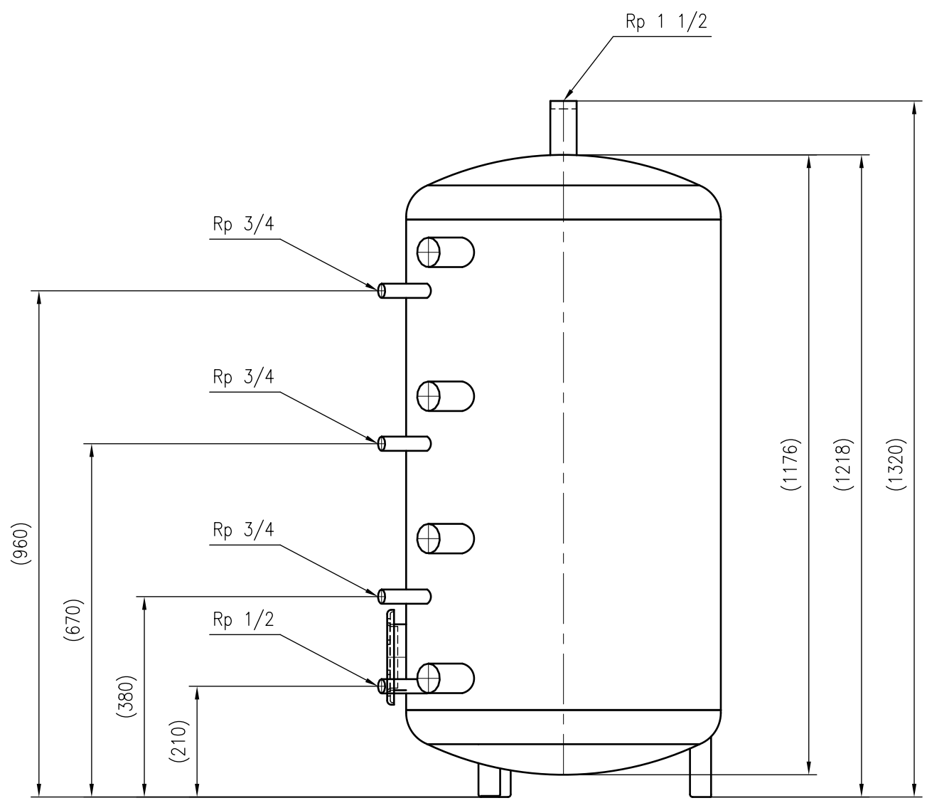
Side view
