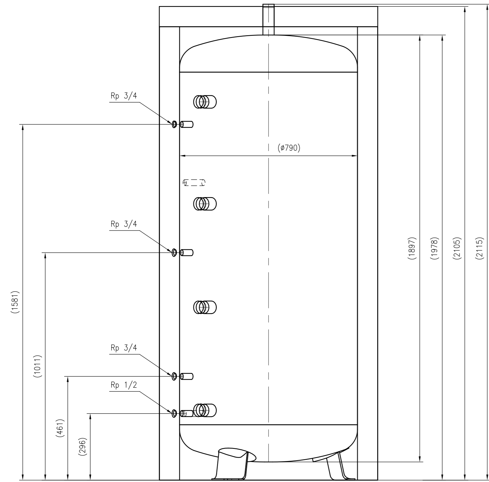
Side view
